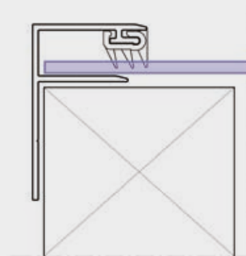
Aluminum F profile available for use where sheet width is reduced, leaving an unsupported edge.
